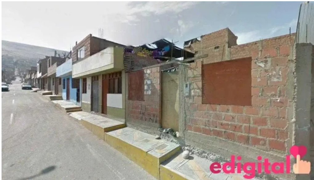
Farmacia tacna
